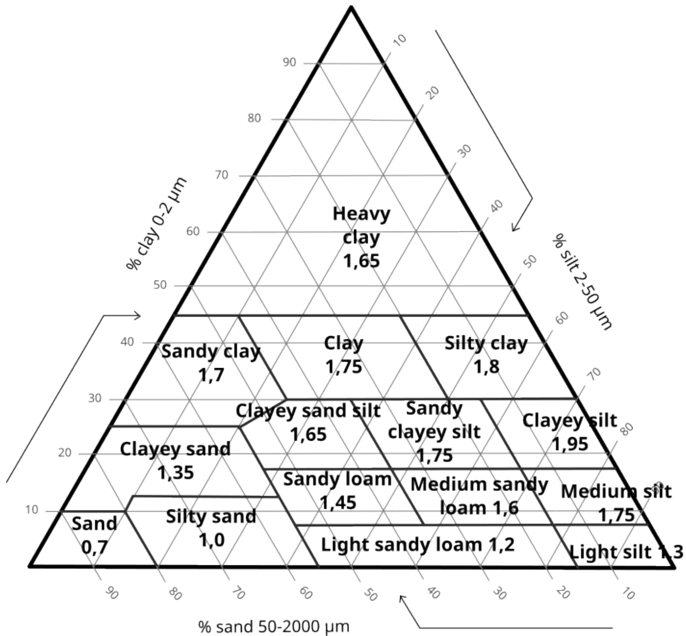
Jamagne's Triangle of Textures (1977) with indication of the available water capacity (AWC) in mm/cm
